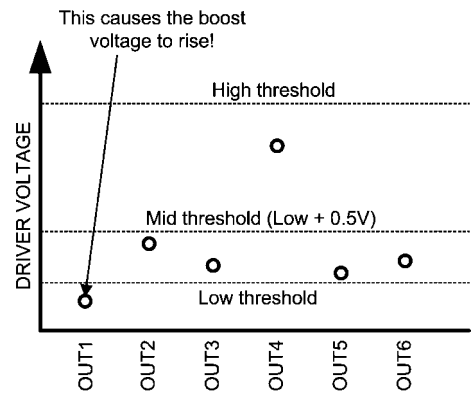
Boost voltage too Low
