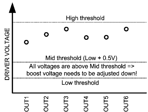
Boost voltage too High
