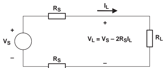
Figure 15. Steady-State Circuit Model
