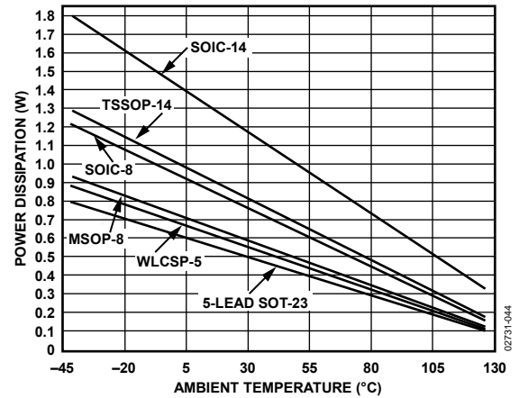
Figure 44. Maximum Power Dissipation vs. Ambient Temperature
