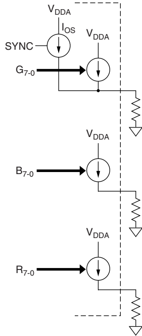
Figure 1. FMS3818 Current Source Structure
