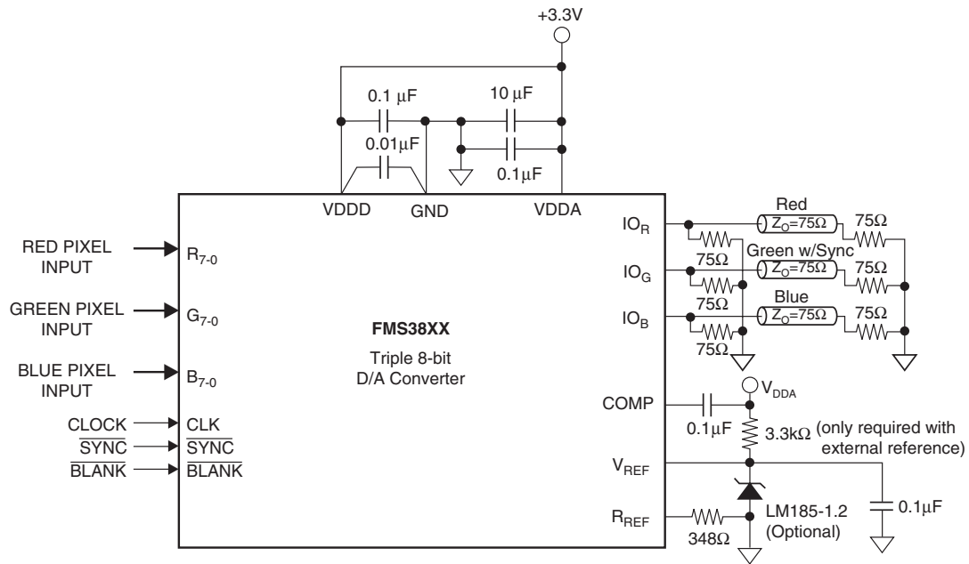
Figure 8. Typical Interface Circuit
