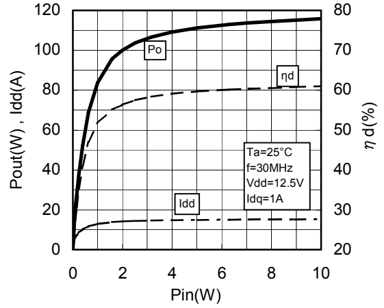
Pin-Po CHARACTERISTICS
