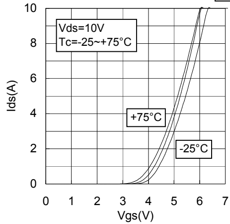
Vgs-Ids CHARACTERISTICS 2
