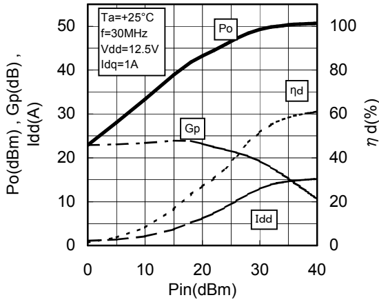
Pin-Po CHARACTERISTICS
