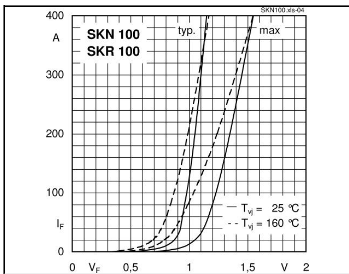
Fig. 5 Forward characteristics
