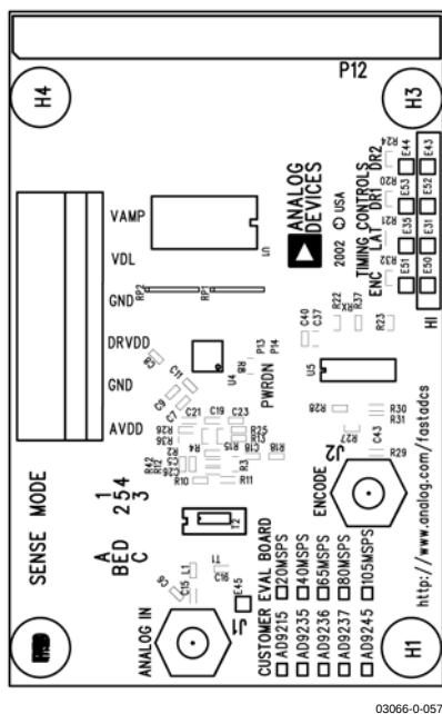
Figure 55. LFCSP Evaluation Board Layout, Primary Silkscreen
