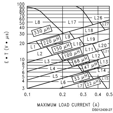
FIGURE 7. LM2594/LM2594HV-ADJ
